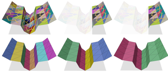
Figure 2: Construction of a hierarchical clustering, as edge collapse of the dual graph merge clusters.
