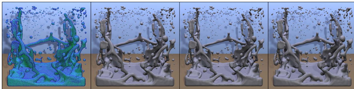
Figure 10: From left: a rendering of the particles inside the generated surface, isotropic constraints, neighbor-based anisotropy and velocity-based anisotropy
