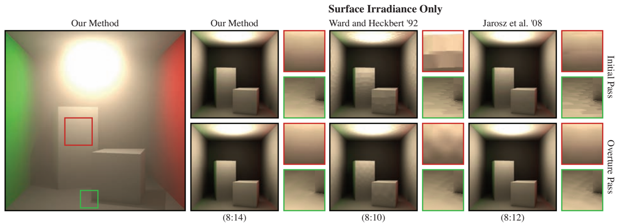
Figure 8: The classic Cornell box scene with a scattering medium. We compare the quality of irradiance caching and provide two zoomed in regions for each result. Ward’s gradient formulation does not consider the medium, which results in inaccurate gradients and significant extrapolation artifacts. The participating media gradients from Jarosz et al. do a much better job, but still suffer from artifacts due to occlusion changes. Our gradients obtain the smoothest results by taking into account the media and occlusions.
