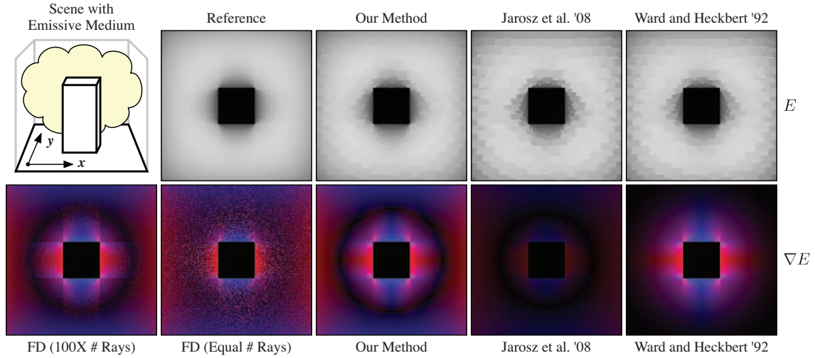
Figure 4: This modification of the scene from Figure 3 contains an emissive medium. Our gradient formulation obtains accurate results by taking into account the medium and surface-medium occlusions, whereas previous methods ignore these effects and suffer from artifacts.
