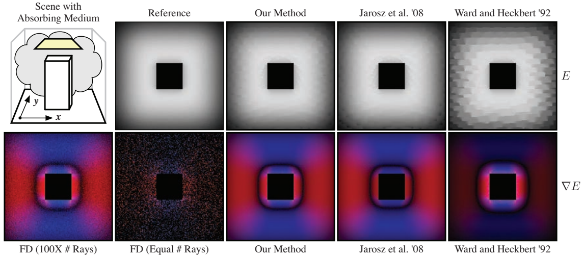
Figure 3: We compare irradiance caching and extrapolation using different gradient computation techniques in a scene with an absorbing medium. The top row shows irradiance extrapolated over the ground plane from a few cache points. Our gradients consider changes of visibility and absorption by the medium. Previous methods, which ignore either visibility [JDZJ08] or absorption by the medium [WH92], lead to increased artifacts. In the bottom row we visualize the irradiance gradients computed per-pixel . The red and blue color coding shows absolute values of the x and y components of the gradient, respectively. We computed gradients for each technique using 1.8K gather rays per pixel and also a “ground truth” gradient using finite differences (FD). Since finite difference gradients are extremely noisy, our reference uses 100 times more rays (180K rays/pixel). Our method produces accurate gradients with few gather rays and converges to the reference solution using finite differencing.
