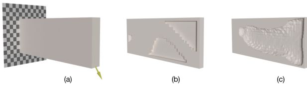
Figure 2: Conventional topology optimization algorithms create internal structures disrupting the inner cavity. Shell structures avoid this problem by adjusting the thickness locally. For a cantilever beam problem (a), example inner structures are shown for (b) conventional topology optimization and (c) shell optimization methods. Note that (b) and (c) are mid-section views.
