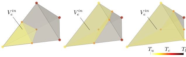
Figure 5: Possible configurations that an element may take an intermediate density value. Color of a vertex indicates its temperature.
