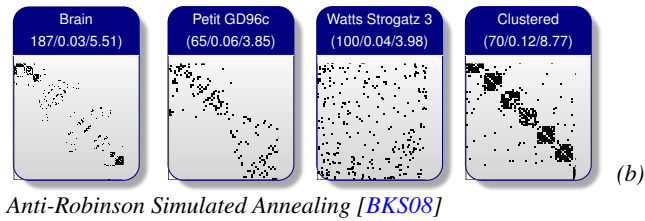
Figure 12: Example for Heuristic Matrix Rearrangings.
