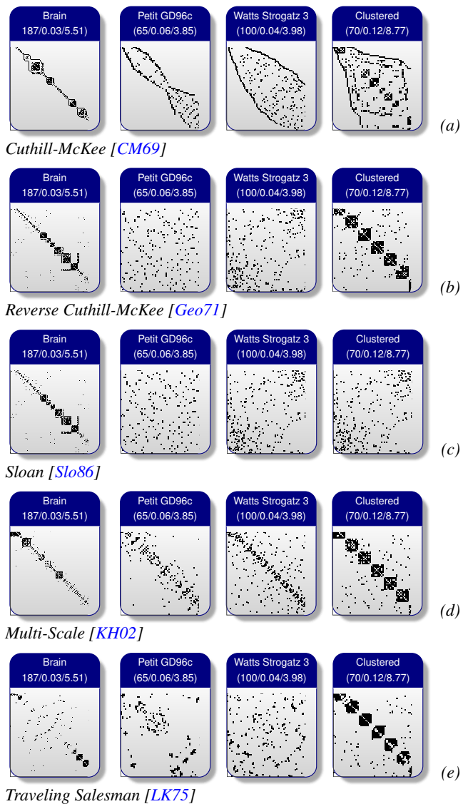
Figure 16: Examples for Graph-based Reordering Approaches.
