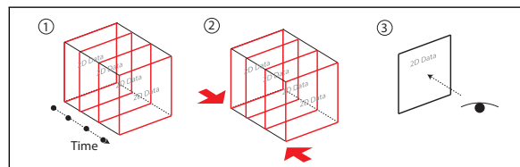
Figure 9: The discrete time flattening operation.
