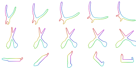
Figure 5: Morphs of tools from [BBBK08]. The correspondence for the pocket knife is given so that the different blades deform from one to the other.
