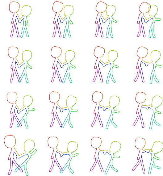
Figure 13: Morphing of the four curves at the corners of the rectangle.
