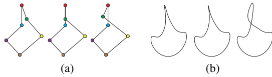
Figure 2: morphs between polygonal curves (a), and C^1 curves (b), with a non-regular intermediate curve.
