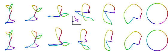
Figure 9: The angle-length method (top) exhibits cusps while our algorithm produces a regular homotopy.
