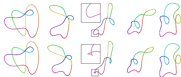
Figure 1: Our morph (top) is guaranteed to be a regular homotopy, while standard methods such as the angle-length method may display cusps as shown in the bottom row.
