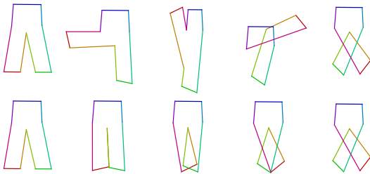
Figure 12: Morphing source and target curves whose turning numbers are one and two respectively. Using the angle-length method directly (top) gives unnatural results. Our automatic choice of the vertex at which flipping should occur (bottom) gives a natural morph.
