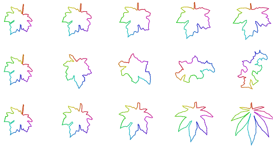
Figure 4: Morphs of leaves from [TvW02]
