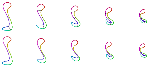
Figure 11: The addition of three diagonals (top) prevents the shrinking of the body of the snake which appears in our regular algorithm (bottom).
