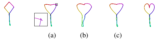
Figure 7: Comparison of (a) angle-length (b) curvature and (c) our algorithm. Note the cusp produced by the angle-length method.
