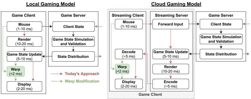
Fig. 11. Late-warp fits in as a modification of the standard gaming models and can substantially reduce motion-to-photon latency for some aspects. Left: Modification to a local gaming model. Right: Modification to a cloud gaming model. The red and green arrows indicate the steps comprising motion-to-photon latency in today’s approach and warp modifications respectively. Note that while input prediction could be used, it adds error, and thus we only evaluate late input latching in this work.
