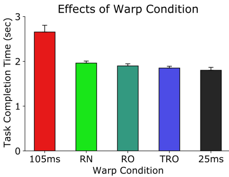
Fig. 8. Effects of warp condition on aiming performance. Bar height is the mean of individual median task completion time in the corresponding warp condition, aggregated across all other factors, and error bars are the standard error of this mean.
