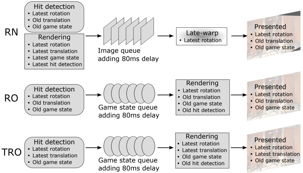
Fig. 7. RN implemented rotational warp by delaying image presentation, and RO and TRO simulated the respective warp methods by delaying game states. Rectangles with sharp edges represent operations on images, and rectangles with rounded edges represent operations on game states. See Sec. 3.4 for details.
