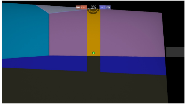
Fig. 6. Missing guard band artifact in RN shown as the black area around the top and right edge. 2D user interface elements (progress indicator at the top and latency measurement box at the right) were added after late-warp and are thus unaffected by the artifact.
