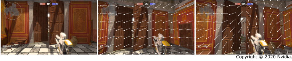
Fig. 2. Visualizing a reprojection in image space. Left : Pre-rendered image. Center : Rotation applied. Right : Translation and rotation applied. Note that the aim changes significantly and some pixels are not in the pre-rendered image.
