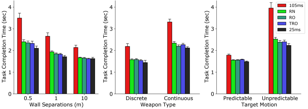
Fig. 10. Effects of wall separation ( Left ), weapon type ( Center ), and target motion predictability ( Right ) on aiming performance. RN , RO , and TRO yielded aiming performance similar to that in 25ms . Error bars represent the standard error of the mean across individual median scores.
