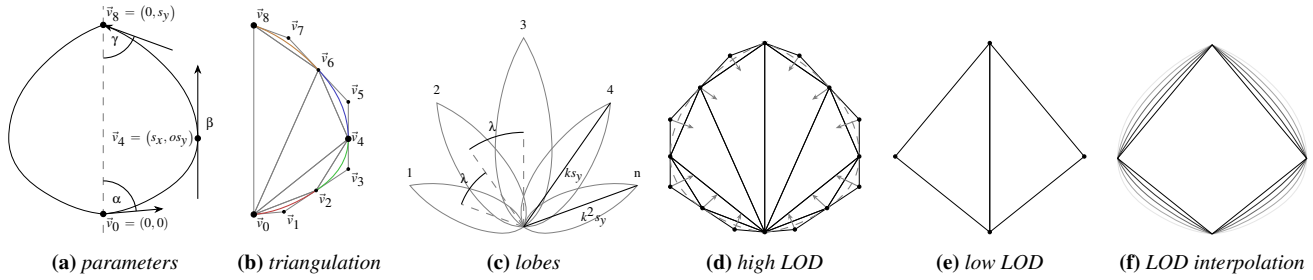
Figure 5: Leaf Geometry. (a) The user defines the lobe shape by the angles (\alpha, \beta, \gamma) , an offset o , or a scale (s_x, s_y) . (b) This results in Bézier curves, shown in different colors, with their corresponding tessellation for later filling the leaf interior. (c) For multilobe leaves, the user defines the lobe count n , the angle between lobes \lambda , and a lobe scale-falloff k . (f) For continuous LOD, we interpolate the (d) high-LOD positions to the edges of the (e) low-LOD.
