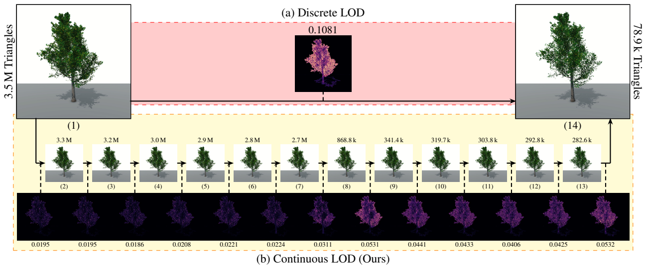
Figure 12: Discrete versus Continuous LOD. (a) shows a conventional, sudden LOD switch from frame (1) to (14) with a high ALIP error. In (b), our method can distribute the change over additional frames (2 – 13), also distributing the visible ALIP error.
