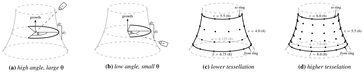
Figure 4: Segment Tessellation. We highlight the forward-facing part of a stem ring for a high (a) and low (b) camera angle. In (c, d), we provide examples with \theta = \frac{\pi}{2} of different fractional tessellation factors and indicate the actual, ceiled tessellation factors in parentheses.
