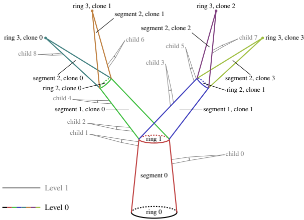
Figure 2: Weber-Penn Model. We mark the different elements of an example tree with two levels. Level 0 splits into four clones.
