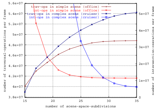
Figure 3: Trading trav-ops vs. int-ops: given any cost-ratio between trav- and int-ops, there is an optimal number of scene-space-subdivisions. However, if this number is not optimally chosen, performance degrades only slowly.
