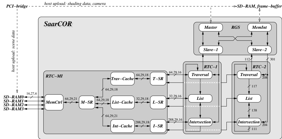
Figure 2: The SaarCOR hardware model splits into three parts: The ray tracing core (RTC), the ray-generation and shading unit (RGS), and RTC’s memory manager (RTC-MI). To allow for easy scaling, several RTCs are supported. Please note the simple routing scheme used: it contains only point-to-point connections and small busses, whose width is also shown separated into data-, address- and control-bits.
