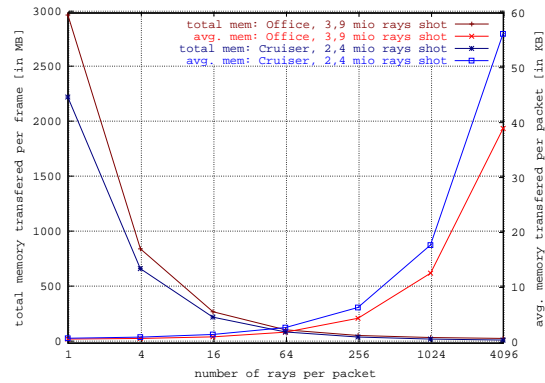
Figure 1: Influence of the number of rays per packet on the amount of memory transferred during rendering of one frame and the average amount of memory requested by a packet. The latter figure gives a rough estimate of the minimum size a cache should have.
