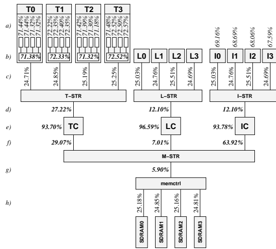
Figure 5: Usage and hit-rates of a standard SaarCOR chip running the BQD-1 benchmark: this shows in detail, that trivial static load-balancing works out perfectly well
