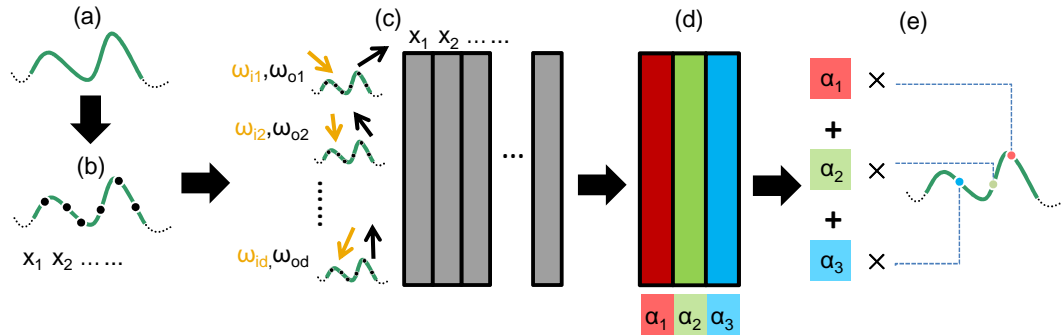
Figure 4: Conceptual diagram for computing characteristic points and weights. The original surface (a) is sampled as a dense point set (b); (c) the reflectance for each point is computed for sampled incident and view directions and then stored in a matrix with one column per sample point and one row per incident/view direction pair; (d) the matrix is approximated by a small subset of columns with associated weights; (e) the filtered reflectance from a dense sampling of points on the original surface is approximated by a weighted sum of reflectance from the points associated with the selected matrix columns.
