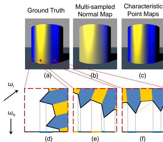
Figure 1: Renderings of a cylinder using different methods. The ground truth (a) is obtained by expensive brute-force multi-sampling. Multi-sampling the simplified geometry with a normal map is shown in (b). Fig. 1(c) uses CPMs. Fig. 1(d-f) are top views of different parts of the original cylinder. The masking effect is shown in (d), and Fig. 1(f) illustrates the shadowing effect, both of which cannot be represented using normal maps and are well preserved by our CPMs. The lighting direction is \omega_l , and the view direction is \omega_o .
