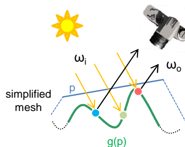
Figure 5: Filtered reflectance reconstruction from characteristic points.
