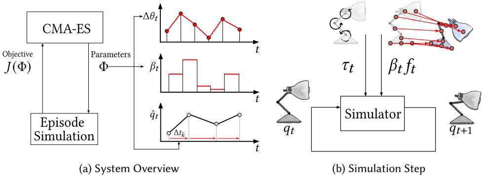
Fig. 2. (a) Visualization of our optimization pipeline, the optimization parameters \Phi , and their interpolation. They correspond to the per-timestep residual PD target \Delta\theta_t , assistive force modulation \beta_t , and the keyframe timings, \Delta t_k . (b) Internal joint actuation and modulated external assistive forces are used in combination.
