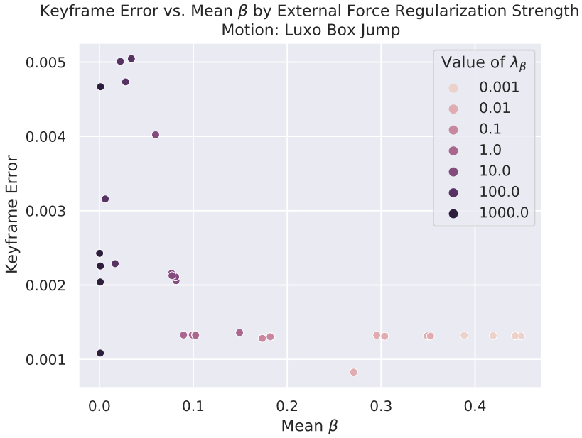
Fig. 14. Comparison of performance across 7 different values of regularization strength \lambda_\beta . Each point represents a solution. Ideal solutions (small assist, small error) reside on the bottom-left corner.
