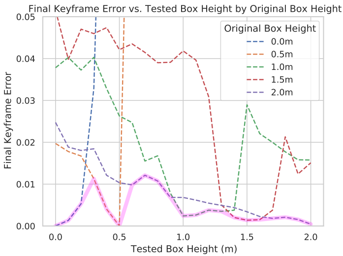
Fig. 11. Deployment performance for solutions learned on different box heights. The best-error envelope is highlighted in a magenta line.
