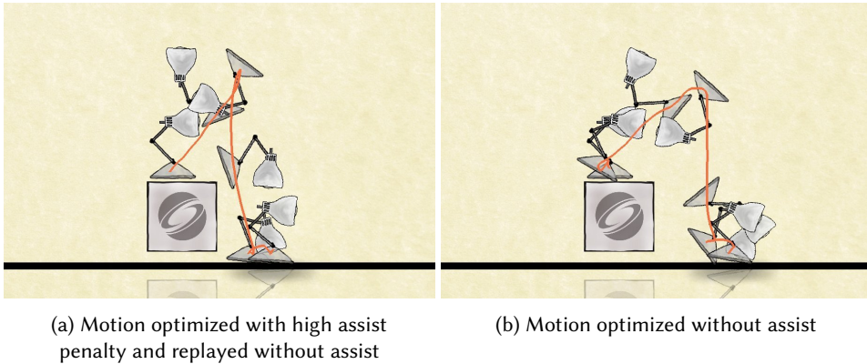
Fig. 9. Comparison of optimized trajectories with and without assist during training. Training with assist yields a more stable trajectory, even with assistive forces disabled at run-time. Note that in (b), the trajectory performs a partial rotation and unstable landing.
