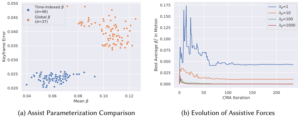
Fig. 6. (a) Comparison of performance between global \beta and time-indexed \beta . Each point represents a solution. Ideal solutions (small assist, small error) reside on the bottom-left corner. (b) Evolution of assistive force usage during optimization, as measured by the mean value of \beta_t^2 used throughout the motion. The optimization initially explores large values of \beta_t and then gradually decreases the reliance on assistive force.
