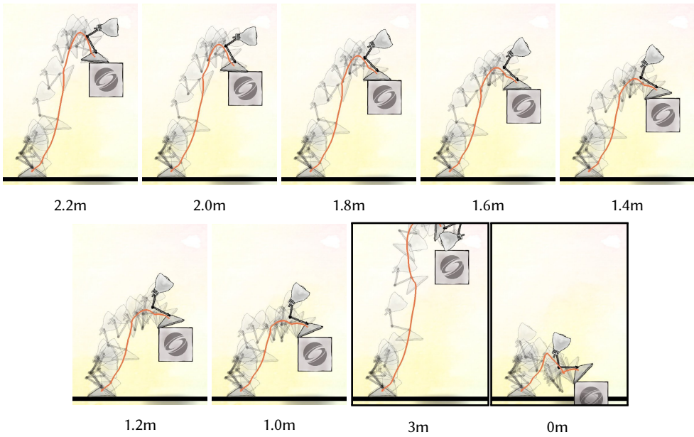
Fig. 10. The converged solution for a particular 2.0m box jump instance is successfully deployed to boxes of other heights without any additional optimization. Outlined scenarios are failure cases.
