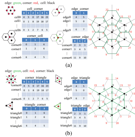
Figure 2: (a): The cell_corner , corner_edge , corner_cell , and edge_corner tables used to represent a 2D Voronoi polygonal grid of climate simulations. (b): The representation of dual triangular mesh of (a). We note that the names of tables and table entries are modified for an illustration purpose in (b), and they are not changed in the real implementation. Thus, from (a) to (b), the content of the four tables keeps intact, which implies that no explicit grid transformation is required.
