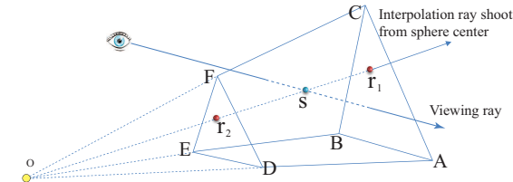
Figure 4: Barycentric interpolation of the scalar value within a triangular frustum. We first interpolate the scalar values at the points \mathbf{r}_1 and \mathbf{r}_2 on the top and bottom triangles, respectively, and then use linear interpolation to compute the scalar value at the point \mathbf{s} on the line segment \mathbf{r}_1\mathbf{r}_2 .
