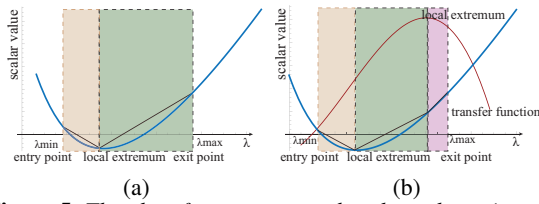
Figure 5: The plot of a reconstructed scalar value using our analytic function. (a) The analytic function is shown in blue, and has one local minimum. The cell along a ray is split into two intervals colored in light orange and green. The analytic function is monotonic within each interval, and its piecewise linear approximation is shown in black. (b) A transfer function is shown in red, and introduces an additional local extremum point. The cell is further split into three monotonic intervals accordingly.
