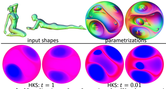
Figure 4: Visualization of surface signals: We show two input shapes from TOSCA’s Victoria category and their parametrization in the top row. In the bottom row we show the mapping of the HKS signals to the sphere for two different timescales, with smaller values drawn in red and larger values drawn in blue.
