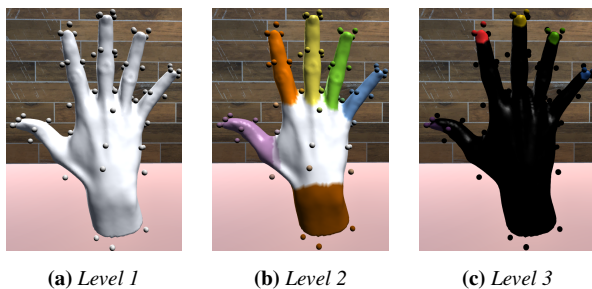
Figure 6: The different levels of the annotation hierarchy; CPs are coloured according to their influence on annotations with threshold 0.4, as described in Section 4.2.2.
