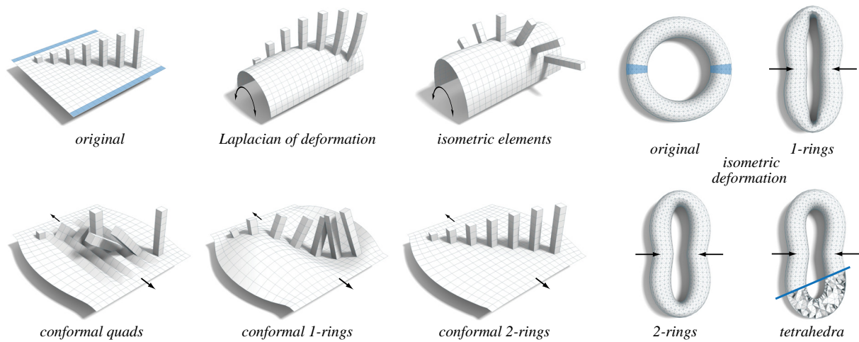
Figure 8: A variety of shape preserving editing tools can be implemented with our framework. Top center: rigid constraints on the polygons lead to intuitive rotations of the protrusions. Bottom left: when stretching the plane with similarity constraints, different deformation behavior is obtained depending on the size and overlap of the elements. Right: comparison of rigid constraints on surface and volume elements. These examples use no smoothing energy or closeness term in Eq. 13, except to define positional constraints for the deformation handles (blue) dragged in the direction of the arrows.
