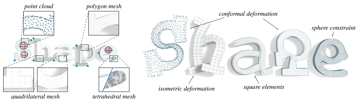
Figure 1: Constraint-based optimization and interactive shape exploration on different geometry representations. Blue dots denote handle positions, green areas are constrained to remain rigid and red spheres indicate that vertices should be arranged on a sphere.
