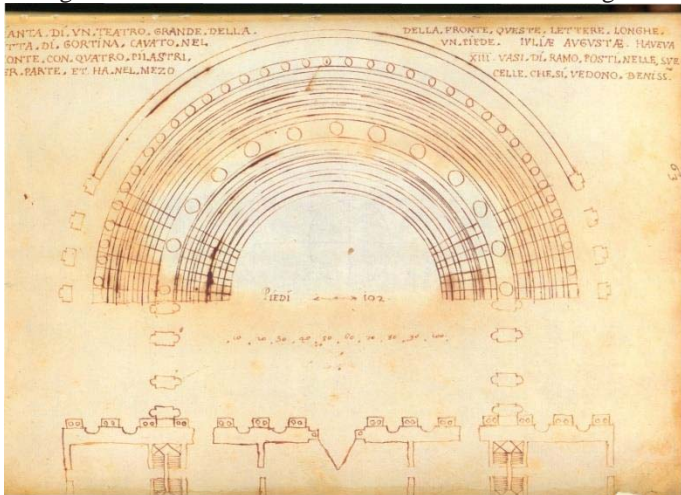
Fig. 1. Plan of the Large Theatre at Gortyn by Onorio Belli. From Beschi L., Onorio Belli a Creta , 1999.
