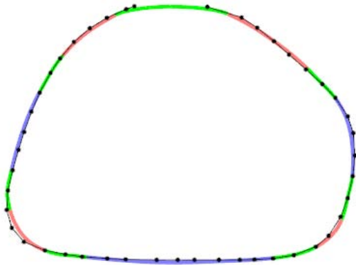
Figure 9: When the endpoints of the input polyline are in close proximity (top of the curve), we close the curve by smoothly interpolating between the two French curve pieces at the endpoints.
