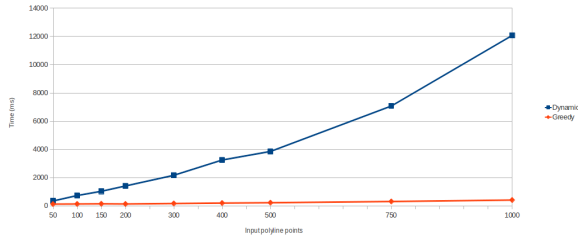
Figure 10: Processing time for our dynamic programming approach compared to a greedy method, for a variety of input sizes.
