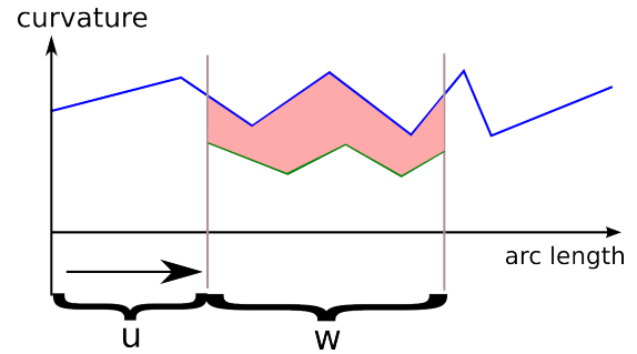
Figure 5: Given the curvature profile of a section of the input curve (green) of length w , we find the optimal curvature fit by sliding it along each of the French curve curvature profiles (blue) and consider using the section of the French curve where the difference (pink) is minimal.
