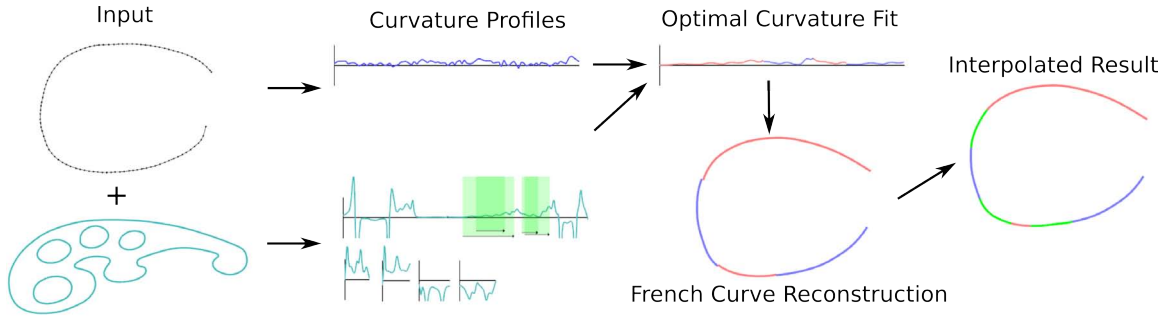
Figure 4: Overview of the algorithm. Curvature profiles are computed for the input polyline and one or more French curves. A dynamic programming algorithm finds sections of the French curve whose curvature profiles optimally match sections of the input curve, while also trying to minimize the number of sections used. The input curve is reconstructed using sections of the French curve with a piecewise clothoid representation. Finally, disjoint sections of the reconstructed curve are interpolated together to produce a connected curve with G^2 continuity.
