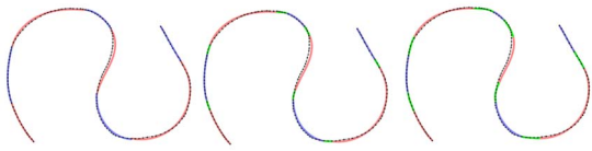
Figure 8: French curve pieces (red and blue) are locally blended with their neighbours (green) using an interpolating function that results in a G^2 curve. The arc-length distance of the blend can be interactively modified. From left to right: 0 (no blend), 10 and 20 units.
