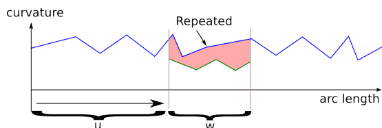
Figure 6: To support closed French curves, we repeat the French curve curvature profile (blue) a second time and slide the window across the point of repetition in order to evaluate all possible sections of the closed curve.
