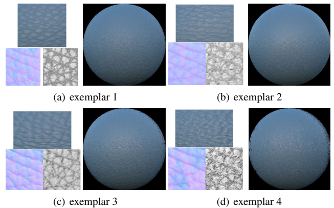
Figure 13: Synthesized mesostructure for the blue faux leather purse given four different input leather exemplars. Top-left: Crop of a sphere rendered with estimated BRDF and given leather mesostructure exemplar. Bottom-left: Synthesized surface normals and specular reflection-occlusion of master tile. Right: Sphere rendered with larger synthesized mesostructure tile.
