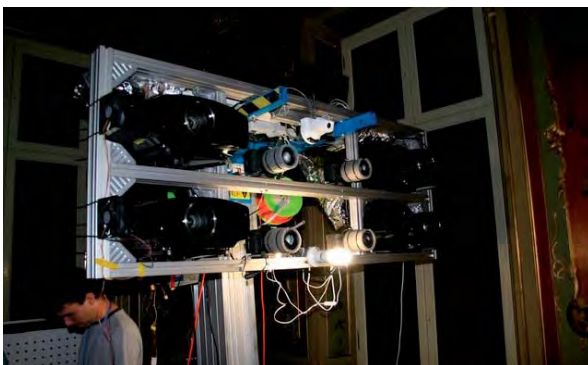
Figure 4: Multidirectional measurement system. This solution speeded up the process of collecting the data thanks to the reduction of indispensable system position changes
