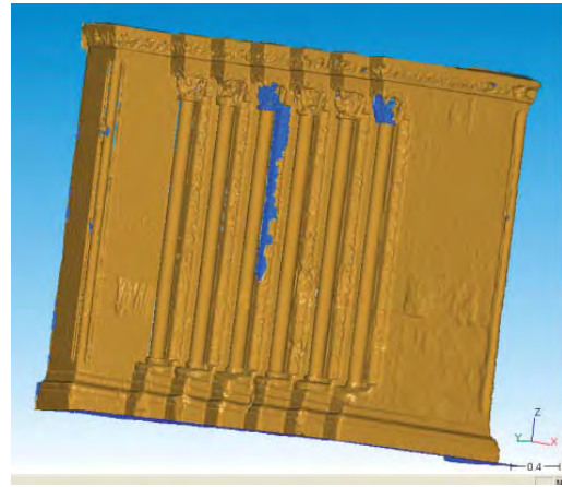
Figure 6: Smoothed mesh
