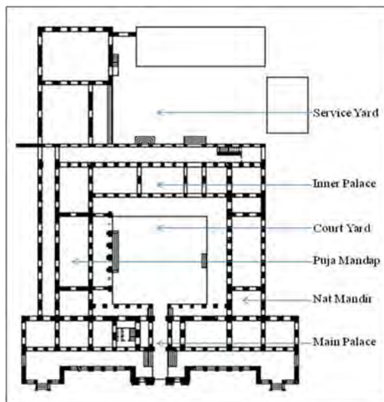
Figure 4: Plan of the Palace
