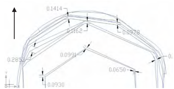
Figure 11: 2D plans from the direct / empirical method (blue line) and laser scanner (black line). For external outline is intended the northern side and for internal the southern one. The measurements indicate the absolute difference comparing the two methods (direct and laser scanner) for some characteristics points of the medieval tower.
