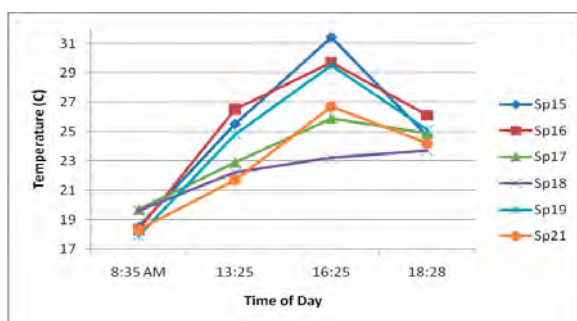
Figure 7: Temperature variations on some of the upper spots on Figure 6
