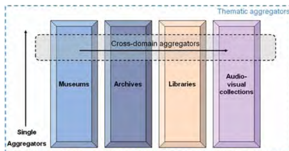
Figure 1: aggregation scenarios
