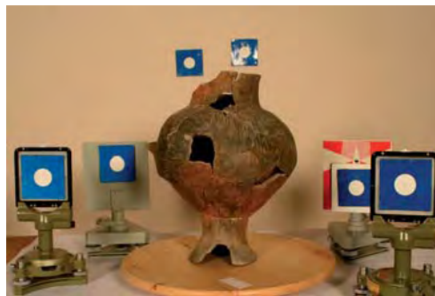
Figure 1: Example of target configuration for different positions of the object
