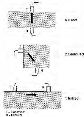
Figure 1: Pulse velocity measurement configurations
