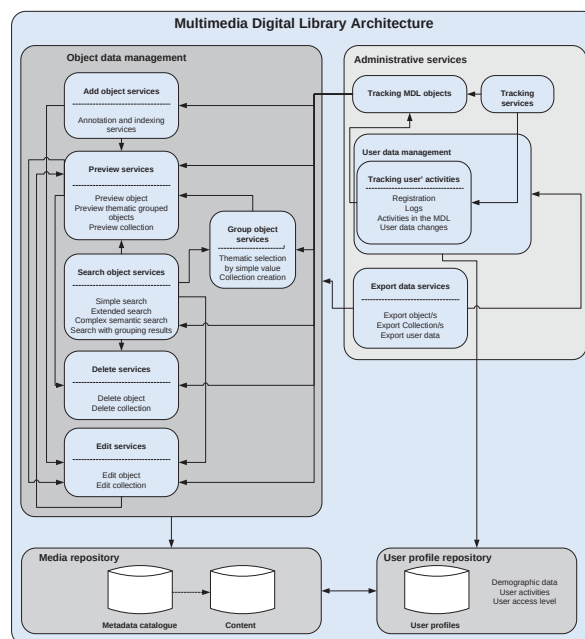
Figure 4: BIDL architecture
