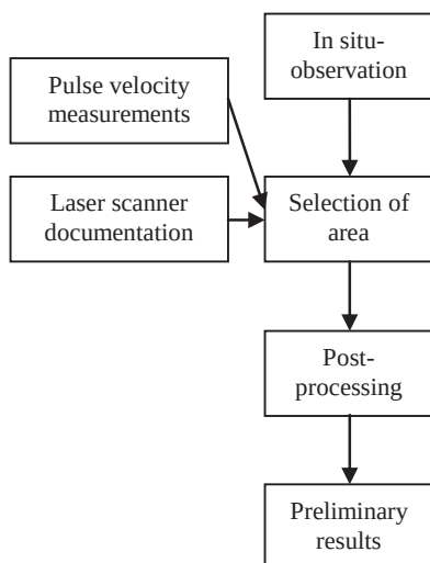
Figure 3: Methodology applied
