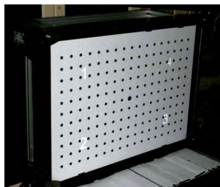
Figure 6: Calibration master for the common calibration
