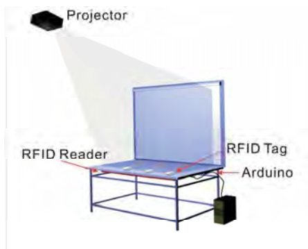
Figure 6: The Framework of the hardware
