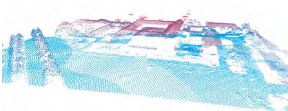
Figure 9: Initial model from airborne laserscan with color indicating height
