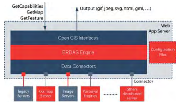
Figure 3: ERDAS APOLLO framework architecture
