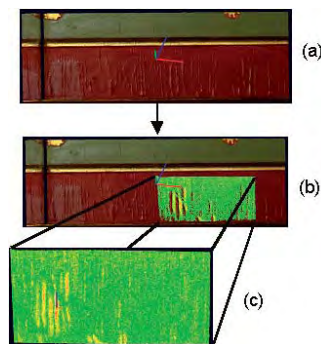
Figure 11: Result of comparison of two measurements: (a) base cloud of points, (b) analyzed cloud of points, (c) result
