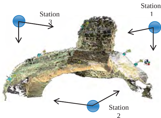
Figure 6: Laser scanning stations at a distance of 10 m from the monument
