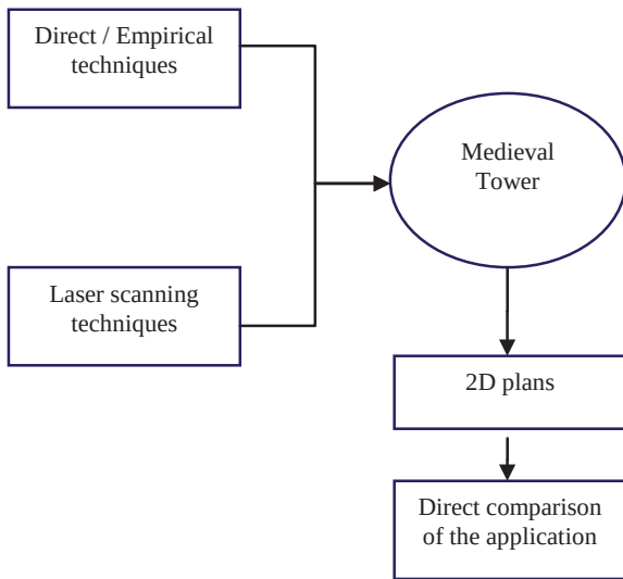
Figure 3: Methodology applied
