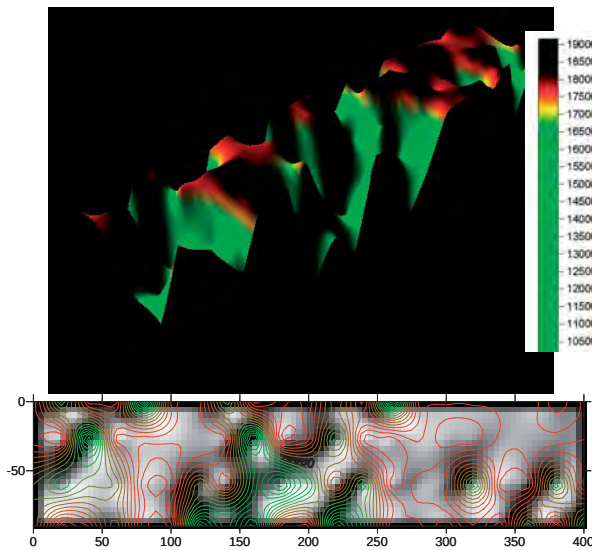
Figure 12: Pulse velocity measurements, presented in different forms in the Surfer software (X-Y axes are cm from the NW corner of the selected area)
