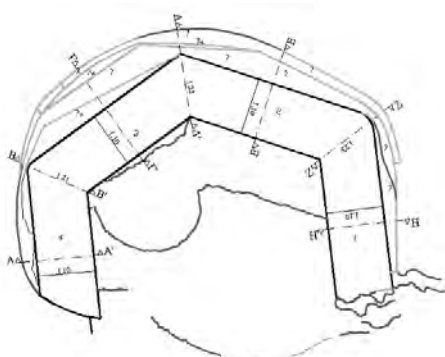
Figure 7: Ground plan and internal facet/view of the four walls
