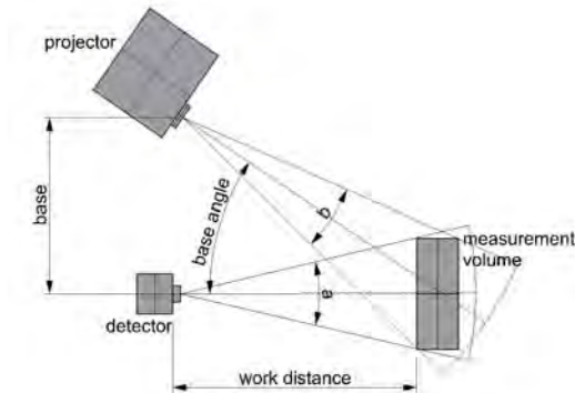
Figure 3: Measurement system setup
