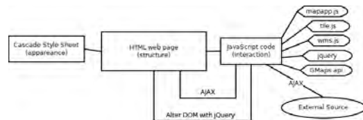
Figure 5: System architecture in the web side
