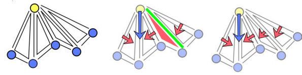
Figure 5: (left) The \epsilon -lower-star and the lower link of a vertex with the height function defined. (center) Algorithm 1 declares the green edge and the red triangle as critical because the edge is not the highest facet of any of its cofacets. (right) Algorithm 2 pairs these cells because the edge is the second highest facet of the unpaired triangle.
