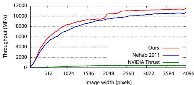
Figure 6: Summed area table.
