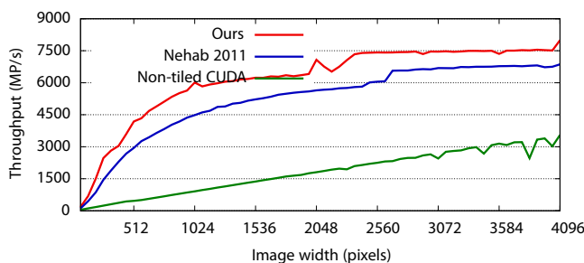
Figure 7: Box filter.
