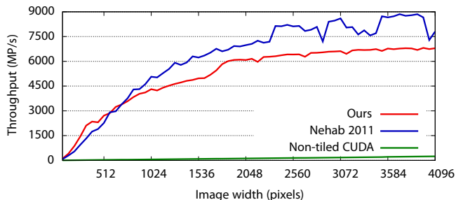
Figure 8: Bicubic interpolation using 1st order causal-anticausal filter pairs. We are an order magnitude faster than a non-tiled implementation but trail Nehab et al. [2011] slightly because we require more shared memory.
