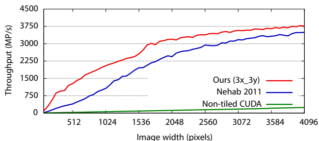
Figure 9: Gaussian blur [van Vliet et al. 1998].
