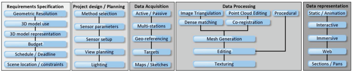
Fig. 1: Overview of a 3D surveying and modelling project: specification definition, planning, data acquisition, processing and representation.
