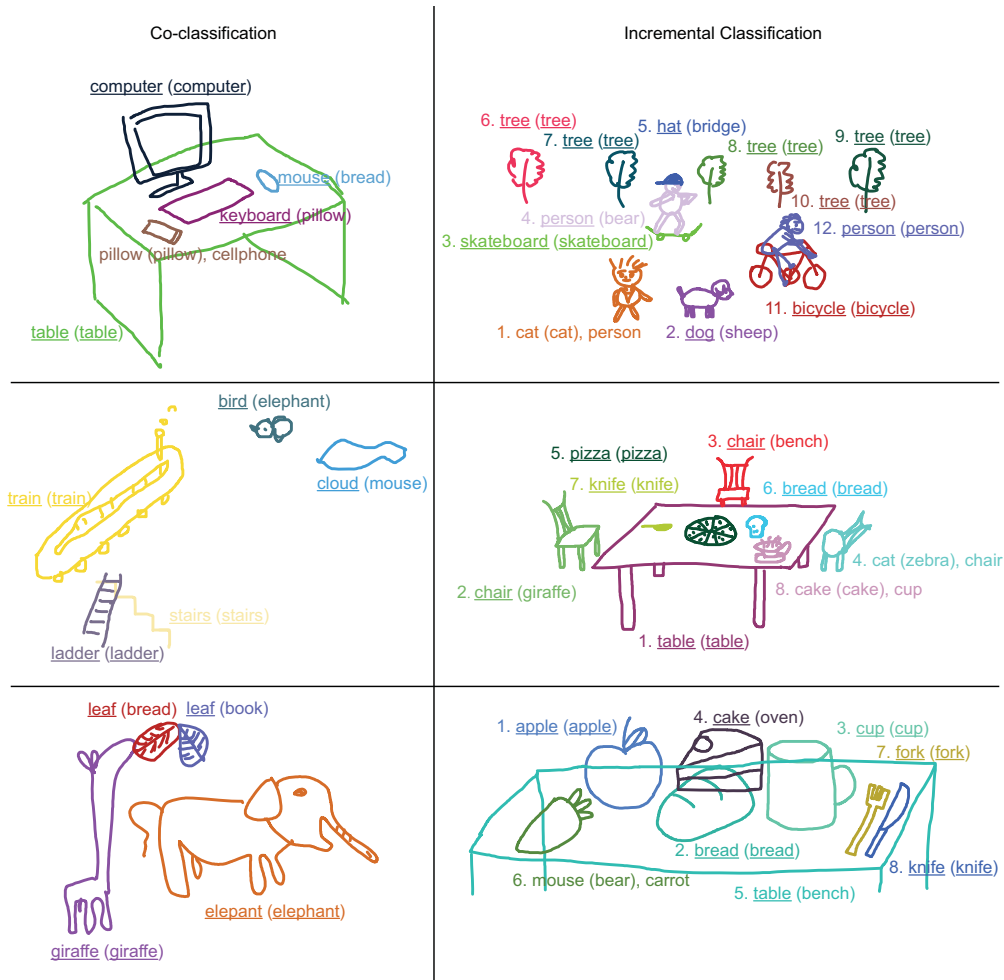
Figure 8: More classification results. Left column: co-classification results; Right column: incremental classification results. The labeled text indicates the prediction of our algorithm and the prediction of the CNN within the parentheses. For incremental classification results, the sequence of drawing is indicated before each label. The underlined labels are consistent with the given ground truth. If none of the predictions are correct, we show the given ground truth at the last.
