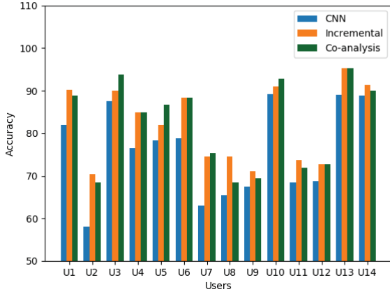
Figure 5: Top-1 Accuracy (%) for sketches drawn by different users.
