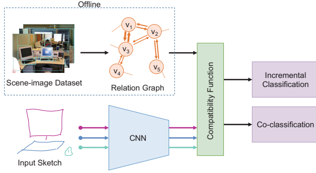
Figure 2: Pipeline of our context-based sketch classification framework.
