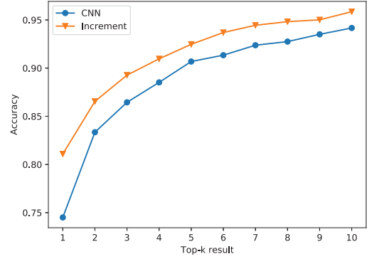
Figure 6: Top-k accuracy (%) of incremental classification.
