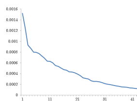
Figure 7: Singular values for the basis in Figure 6.
