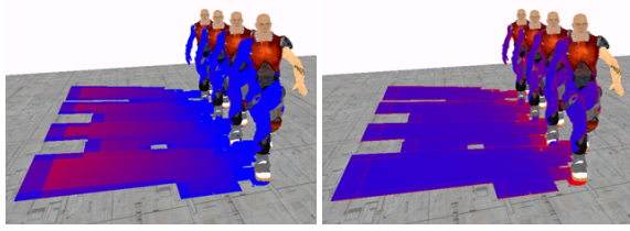
Figure 5: Illustration of the kernel size (left) and coherence (right). Blue indicates a small value, while red indicates a large value. Pixels with zero sized kernel are rendered with shading and textures.
