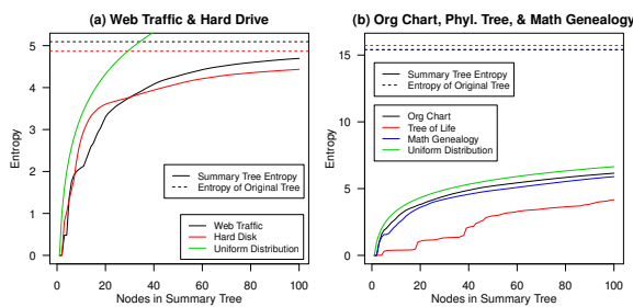
Figure 6: Entropy profiles for k = 1, \dots, 100 for all 5 data sets. For the web traffic and hard drive data sets, the (approximate) maximum entropy summary trees have nearly as high entropy as the original trees using many fewer nodes.
