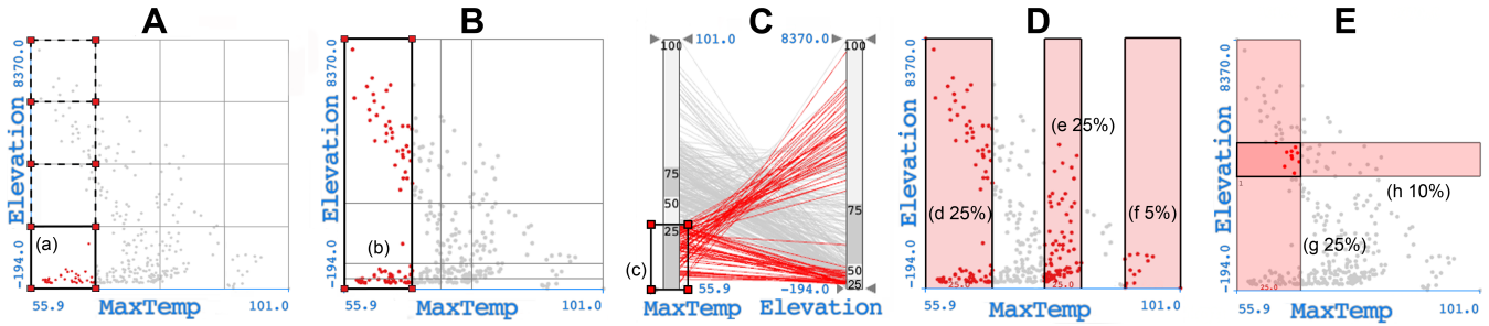
Figure 1: Overview of the extensions for structured brushing. A: A scatterplot with a regular 4 \times 4 grid (value-based). The constrained brush (a) is moved vertically across 4 predefined intervals. The initial position and all consequent positions (dashed brushes) are shown. B: A scatterplot with a percentile 4 \times 4 grid (rank-based). C: Parallel coordinates with a one-dimensional “quartile grid” enabled for both axes. The brush (c) is placed over the first strip of the grid (compare (c) with the brush (b)). D: A scatterplot with three percentile brushes with respect to the horizontal dimension. E: The two percentile brushes are combined using a logical AND operation. The user can grab the intersection and move both brushes.
