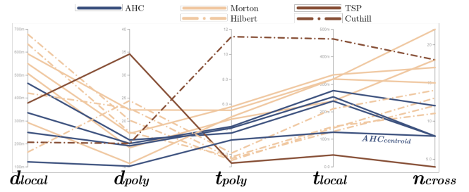
Figure 7: PCP plot showing the global ( d_{poly} & t_{poly} ), as well as local scores ( d_{local} , t_{local} & n_{cross} ), obtained using the interactions visible in Figure 4 (⑤ & ④)) for different orderings for the NYC dataset.
