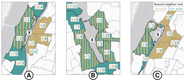
Figure 2: Neighborhoods and nearest neighbor ranks of polygons ( x ) determined by contiguous borders (■) and fixed k ( =6 ) nearest neighbors (■). ■ consider only neighbors on the same side of obstacles like rivers (A) & (C) and prevent underestimation (B) or overestimation (C) when the number of contiguous neighbors differs from k .
