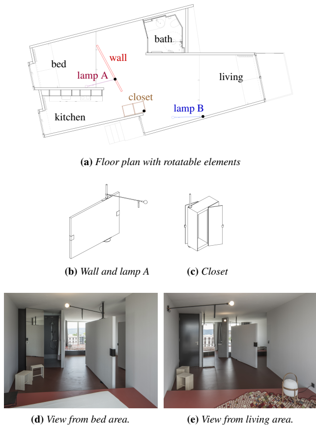
Figure 1: A floor plan of the Mock-up shows the four rotatable elements all at zero degree angle as defined by the sensors and with different colors. Red for wall, brown for closet, purple for lamp A and blue for lamp B. Centers of rotation are shown as black circles.
