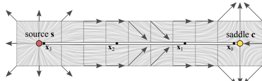
(a) Construction of a simple vector field on a 12 \times 3 grid with a source, a saddle and a full separatrix in between. Velocity is interpolated bilinearly.
