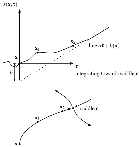
Figure 2: [FRT15] Behavior of s(\mathbf{x}, \tau) for a separatrix.
