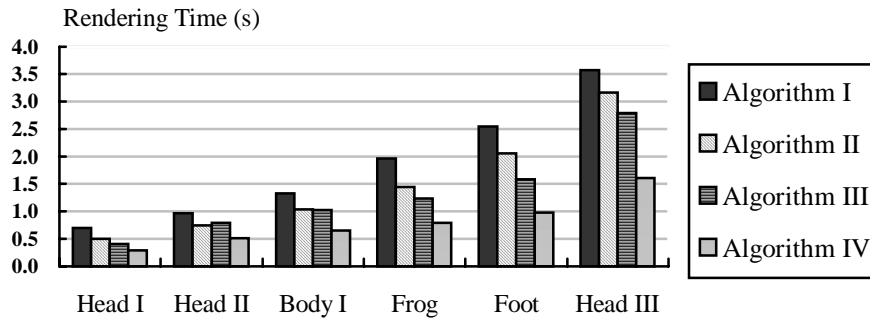
Fig. 7. The rendering time of four algorithms
