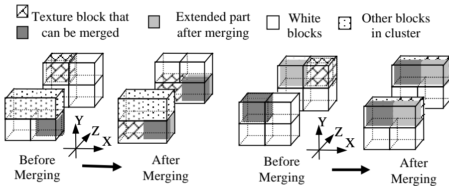
Fig. 5. Two examples of merging between clusters
