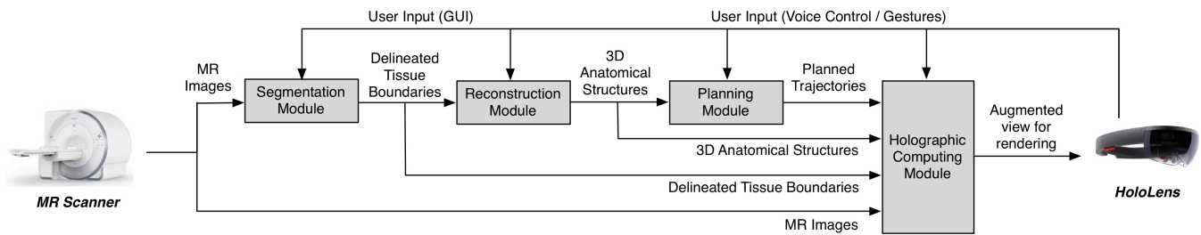
Figure 2: Architecture of the computational core showing its modules and the flow of data and commands
