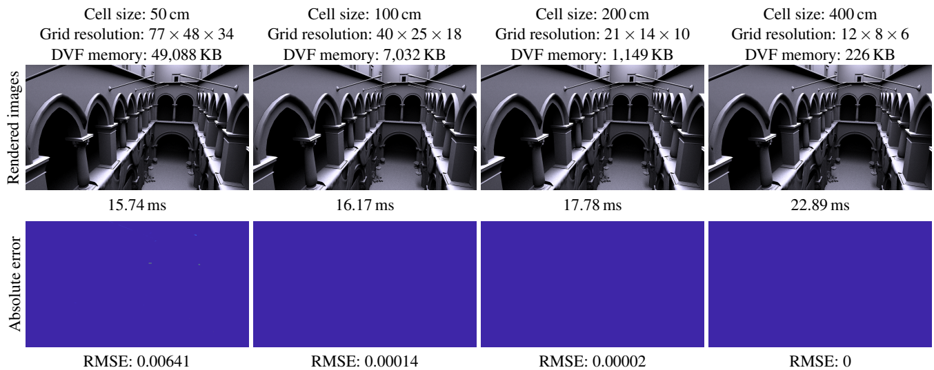
Figure 7: Comparison of the rendering results without textures in the Crytek Sponza scene using DVFs with different cell sizes. From left to right: 50, 100, 200, and 400 cm. Upper row: rendering results of our method. Lower row: absolute error between rendered images with and without DVFs.
