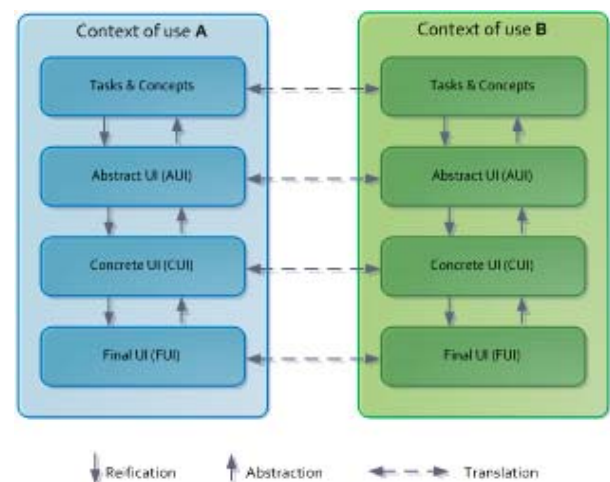
Figura 1: Framework Cameleon.
