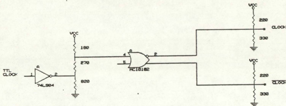
Fig.9 - Interfacing the BT458 to the TTL clock
