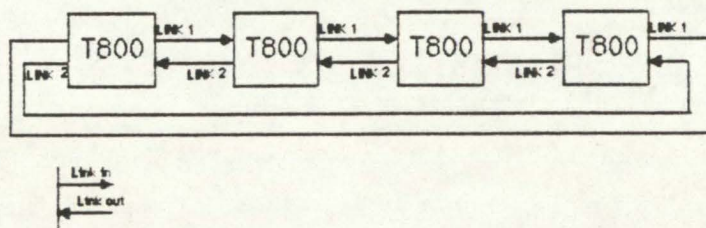
Fig. 2 - Transputers in a ring network
