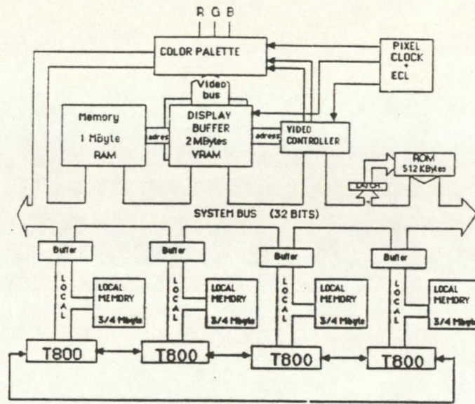
Fig.3 - Blocks diagram of the graphics system.
