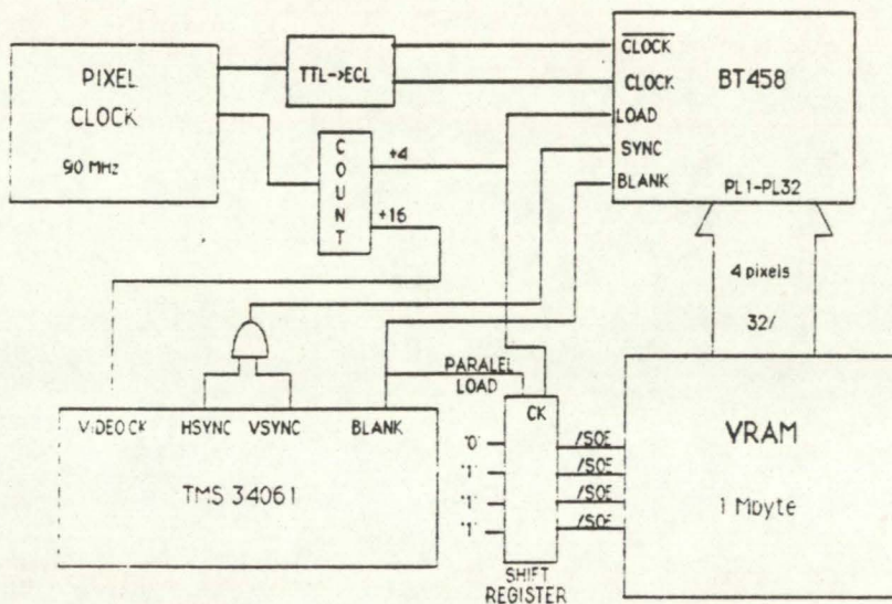
Fig. 8 - Functional block diagram of video output hardware
