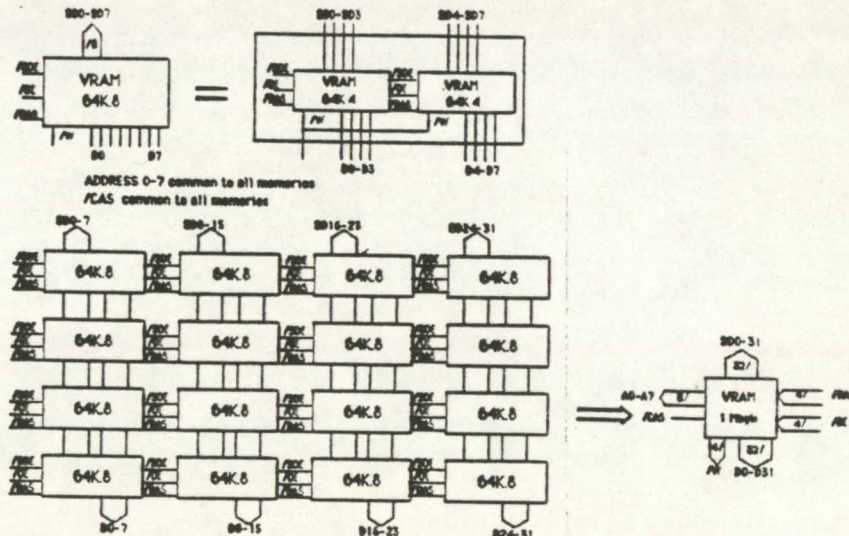
Fig. 7 - Frame buffer organization
