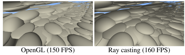
Figure 6: OpenGL with tessellation level 12 \times 12 vs. primary ray casting. Although no tessellation artifacts are visible and shading normals are continuous, frame rates with ray casting are even higher on a GeForce RTX 2080 GPU than with rasterization.
