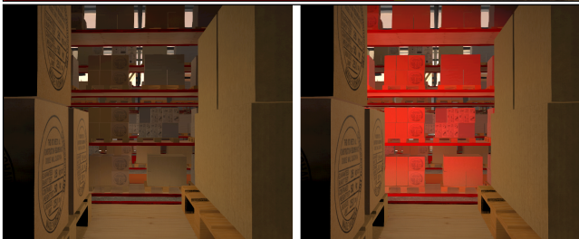
Figure 15: Single-layer shading misses the indirect bounce off the red floor (bottom left), yielding inconsistent shading in WAREHOUSE; using two layers (bottom right) corrects this.
