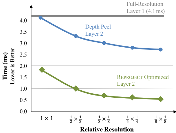
Figure 11: Performance of two methods for generating the Deep G-buffer’s 2nd layer vs. resolution in SPONZA. Our REPROJECT algorithm is twice as fast as traditional DEPTHPEEL. As the resolution for the second layer decreases, the incremental cost of generating a second layer with REPROJECT asymptotically drops to only 25% of that of the first layer, a 4x savings over naive depth peeling.
