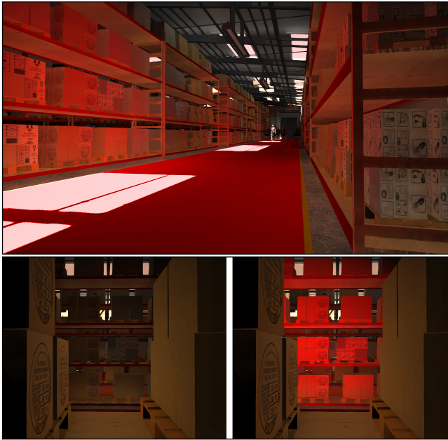
Figure 15: Single-layer shading misses the indirect bounce off the red floor (bottom left), yielding inconsistent shading in Warehouse ; using two layers (bottom right) corrects this.
