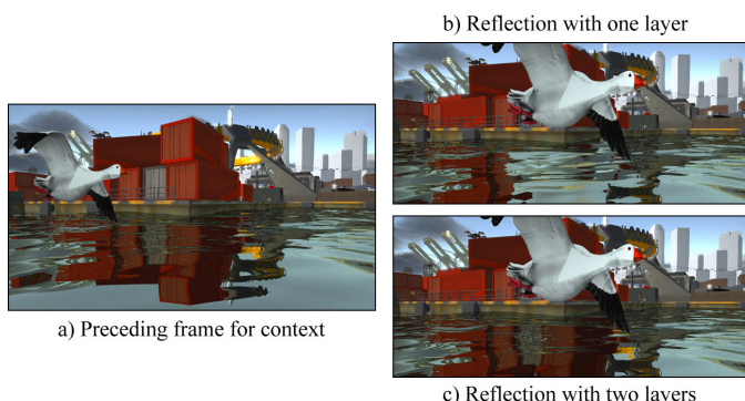
Figure 13: A second layer makes the red containers' reflection in Dockside more stable to passing foreground objects.
