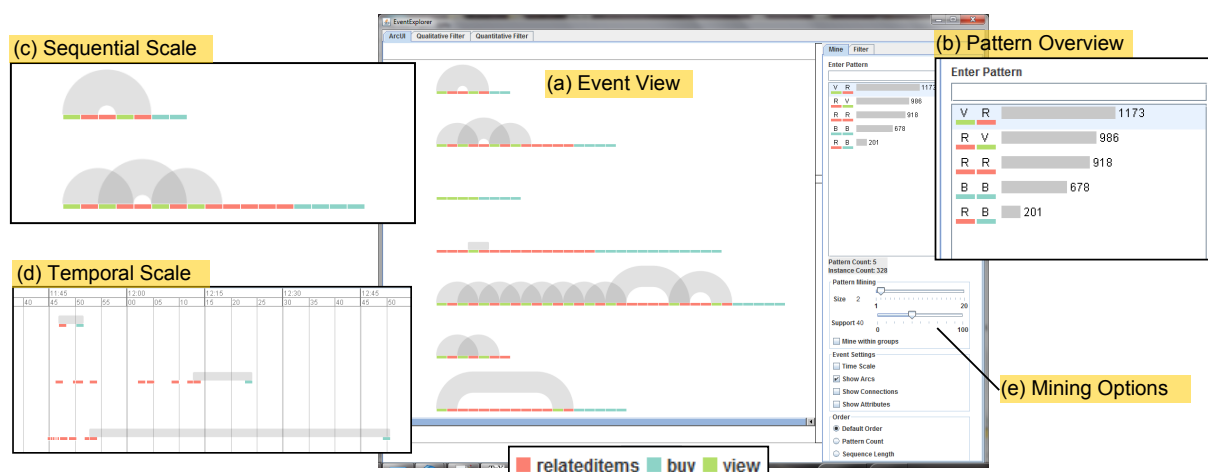
Figure 1: Interface. (a) Events of a case are shown as a horizontal sequence of bars. Cases (event sources) are arranged vertically. Recurring instances of the selected pattern are connected by arcs. (b) A vertical bar chart shows pattern frequency. (c) Sequential scaling. (d) Temporal scaling emphasizes the actual time of events.
