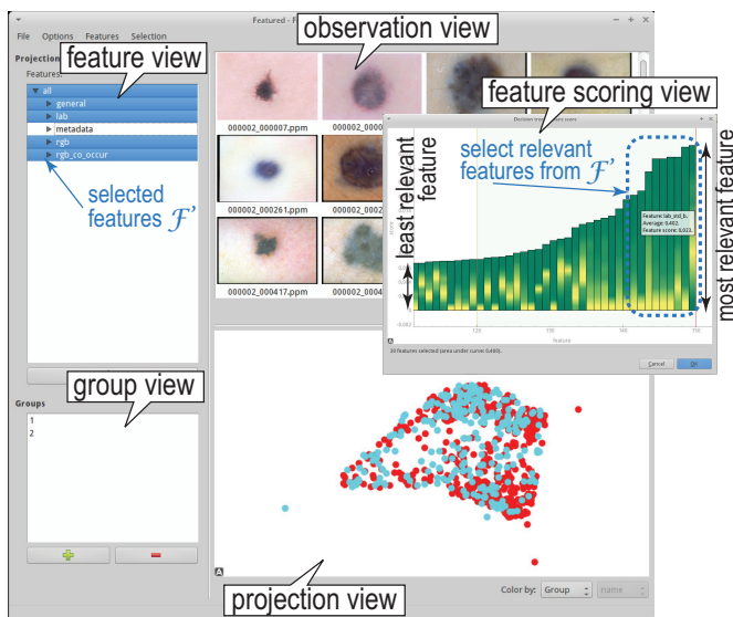
Figure 1: Tool overview
