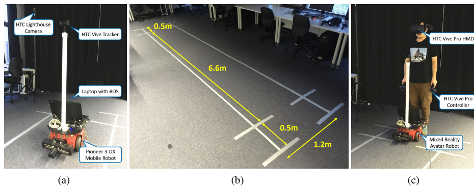
Figure 1: Hardware setup, environment and participant: (a) Mixed-reality avatar robot consisting of an HTC Vive tracker, a laptop running Robot Operating System (ROS) and a Pioneer 3-DX mobile robot. (b) The experimental environment. (c) Ready state of participant and robot in the task "walking following an avatar robot".
