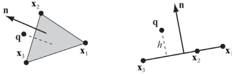
Figure 7: Constraint function C(\mathbf{q}, \mathbf{x}_1, \mathbf{x}_2, \mathbf{x}_3) = (\mathbf{q} - \mathbf{x}_1) \cdot \mathbf{n} - h makes sure that \mathbf{q} stays above the triangle \mathbf{x}_1, \mathbf{x}_2, \mathbf{x}_3 by the cloth thickness h .
