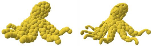
Figure 28: The rotation information of oriented particles cannot only be used to stabilize shape matching, it also allows the use of ellipsoids as collision primitives. The figure shows how the same mesh is approximated much more accurately with ellipsoids (right) than with the same number of spheres (left).
