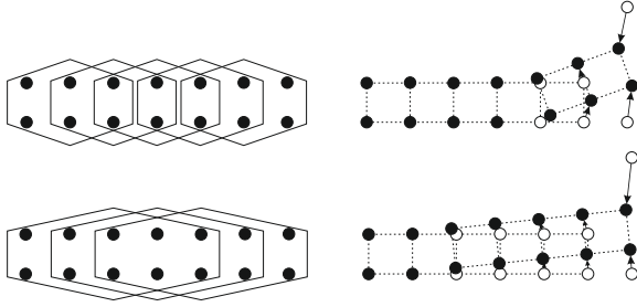
Figure 25: The stiffness of the model depends on the region size. Smaller regions (top) allow larger deformations than larger regions (bottom). The hexagons in the left images represent the overlapping regions of the model. The right images show the goal positions after one particle is moved away.
