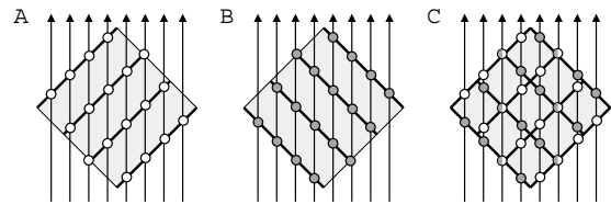
Figure 13: Abrupt change of the location of sampling points, when switching from one slice stack (A) to another (B).
