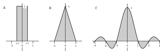
Figure 2: Three reconstruction filters: (a) box, (b) tent and (c) sinc filters.
