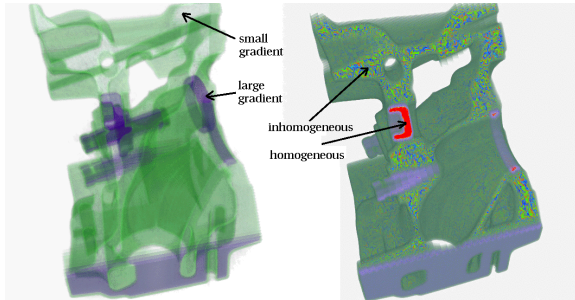
Figure 40: Gradient-weighted opacity allows to identify regions of big variation in the data (left), while high-frequency transfer functions allow to identify small variations (right). Note, that homogeneous and inhomogeneous regions inside the engine data set can easily be identified.
