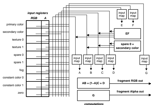
Figure 8: The final combiner stage of NVIDIA's register combiner unit.
