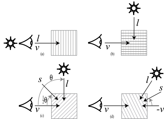
Figure 28: Modified slicing approach for light transport computation.
