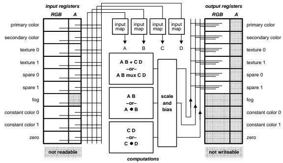
Figure 7: A general combiner stage of NVIDIA's register combiner unit.
