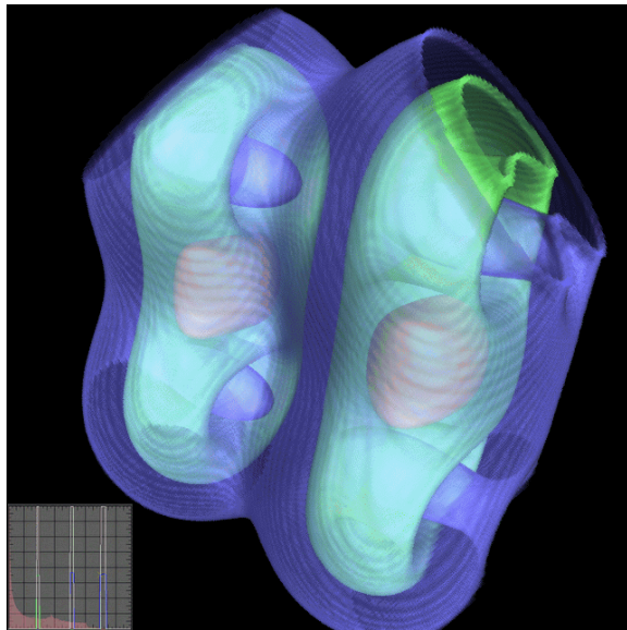
Figure 43: Visualization of iso-surfaces using transfer function peaks (bottom, left) and pre-integrated shaded volume rendering does not lead to holes in the iso-surfaces for a low number of slices as opposed to post-classification.
