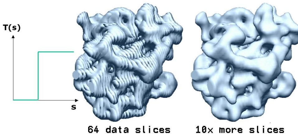
Figure 20: A step in the transfer function or an alpha test GL\_EQUAL generates a single-sided iso-surface. Note, that the artifacts in the iso-surface are removed by very high sampling rates.
