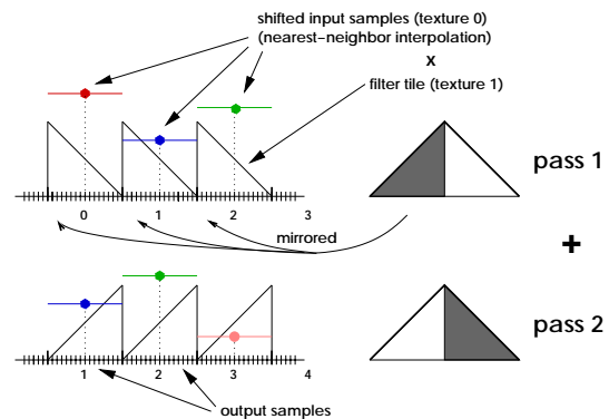
Figure 34: Tent filter (width two) used for reconstruction of a one-dimensional function in two passes. Imagine the values of the output samples added together from top to bottom.
