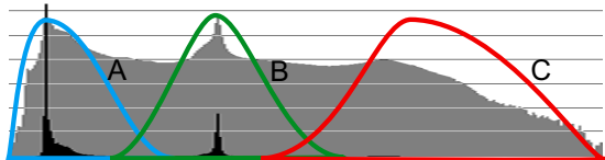
Figure 29: A 1D histogram of the CT human head data set (black: log scale, grey: linear scale). The colored regions (A,B,C) identify basic materials.
