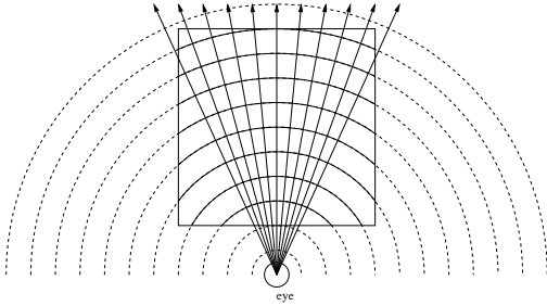
Figure 19: Shell rendering provides a constant sampling rate for all viewing rays.
