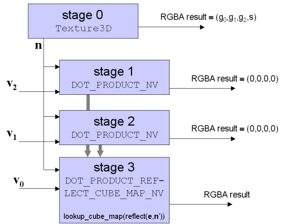
Figure 25: Texture shader configuration for lookup into a reflection cube map. For a diffuse cube map lookup, the last fetch operation is replaced by a DOT_PRODUCT_TEXTURE_CUBE_MAP_NV operation.
