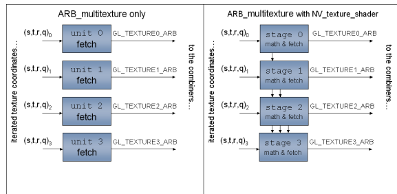
Figure 6: Comparison of traditional multi-texturing and multi-texturing using NVIDIA's texture shader concept.
