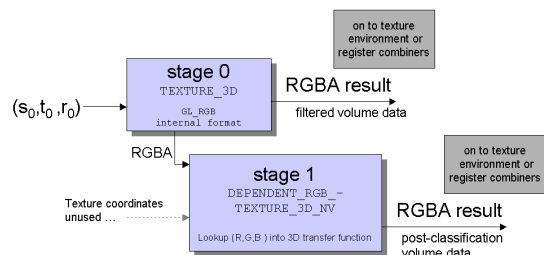
Figure 32: Texture shader setup for a three-dimensional transfer function. Stage 0 fetches the per-voxel scalars while stage 1 performs a dependent texture lookup into the 3D transfer function.
