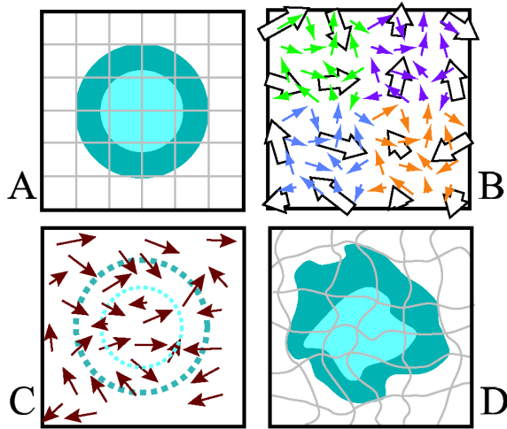
Figure 46: An example of texture coordinate perturbation in 2D. A shows a square polygon mapped with the original texture that is to be perturbed. B shows a low resolution perturbation texture applied to the polygon multiple times at different scales. These offset vectors are weighted and summed to offset the original texture coordinates as seen in C. The texture is then read using the modified texture coordinates, producing the image seen in D.
