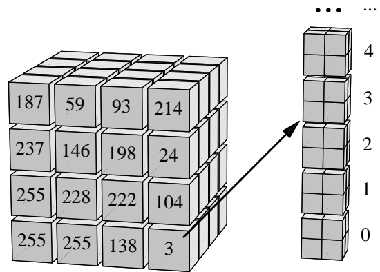
Figure 44: Data structure for vector quantization of volume textures. Each byte of the index data specifies one data block consisting of 2 \times 2 \times 2 voxels.
