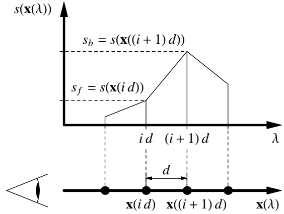
Figure 36: Scheme of the parameters determining the color and opacity of the i -th ray segment.
