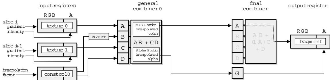
Figure 15: Register combiners configuration for the interpolation of intermediate slices.
