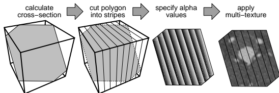
Figure 16: Interpolation of view-aligned slices by rendering slab-polygons.
