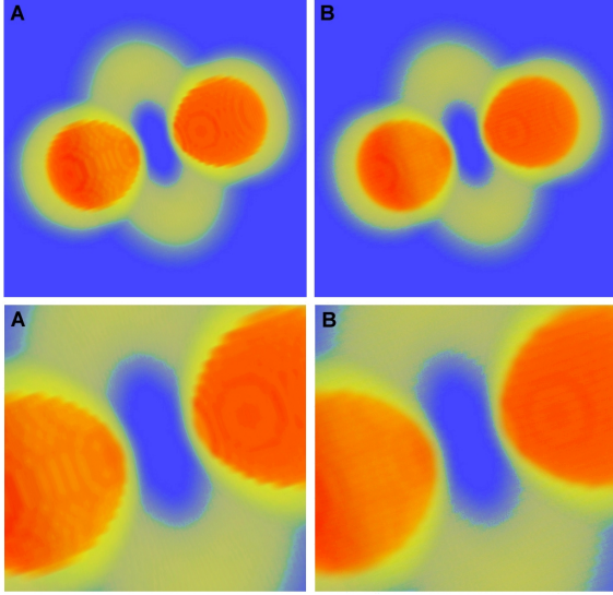
Figure 35: Using a high-quality reconstruction filter for volume rendering. This image compares bi-linear interpolation of object-aligned slices (A) with bi-cubic filtering using a B-spline filter kernel (B).
