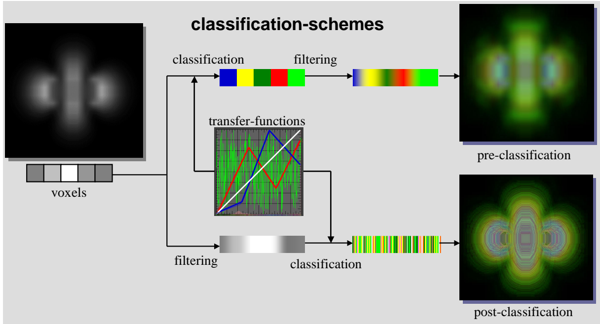
Figure 3: Comparison of pre-classification and post-classification. Alternate orders of classification and filtering lead to completely different results. For clarification a random transfer function is used for the green color channel. Piecewise linear transfer functions are employed for the other color channels. Note, that in contrast to pre-classification, post-classification reproduces the high frequencies contained within in the transfer function.
