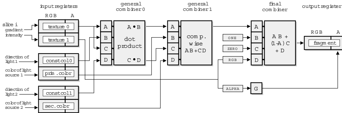
Figure 22: NVidia register combiner setup for diffuse illumination with two independent light sources.
