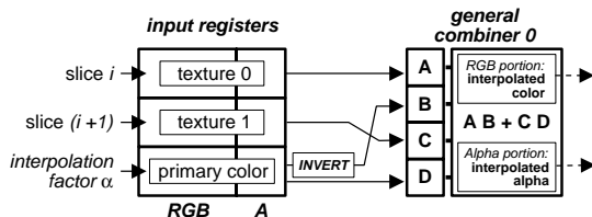
Figure 17: Register combiners configuration for rendering tri-linearly interpolated stripe polygons.
