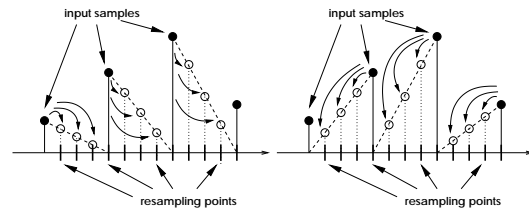
Figure 33: Distributing the contributions of all “left-hand” (a), and all “right-hand” (b) neighbors, when using a tent filter as a simple example for the algorithm.
