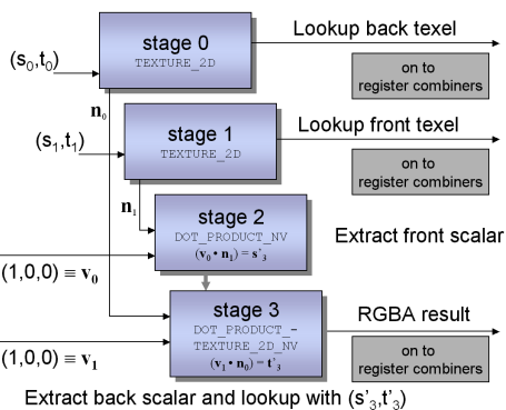
Figure 38: Texture shader setup for dependent 2D texture lookup with texture coordinates obtained from two source textures. If 3D textures are employed, the first two fetch operations are replaced by the corresponding 3D texture fetches.
