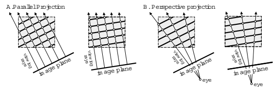
Figure 18: For perspective projections the sampling rate varies for each viewing ray (left: parallel projection, right: perspective projection).
