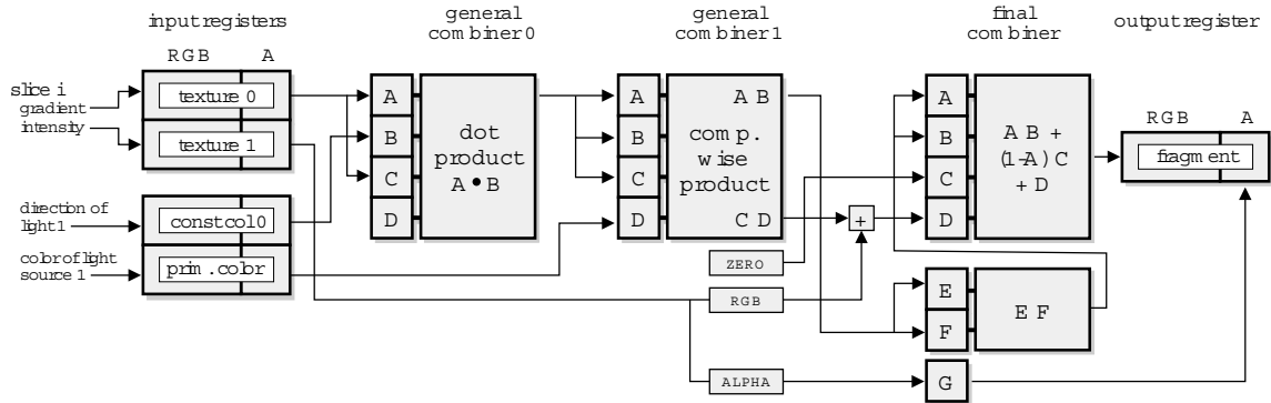
Figure 23: NVidia register combiner setup for diffuse and specular illumination. The additional sum (+) is achieved using the spare0 and secondary color registers of the final combiner stage.
