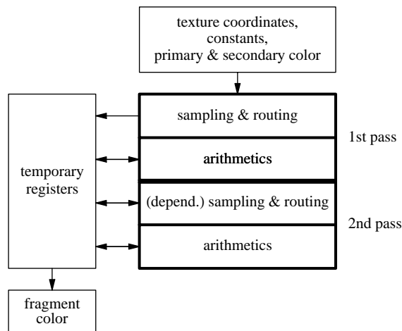
Figure 9: The ATI fragment shader unit.
