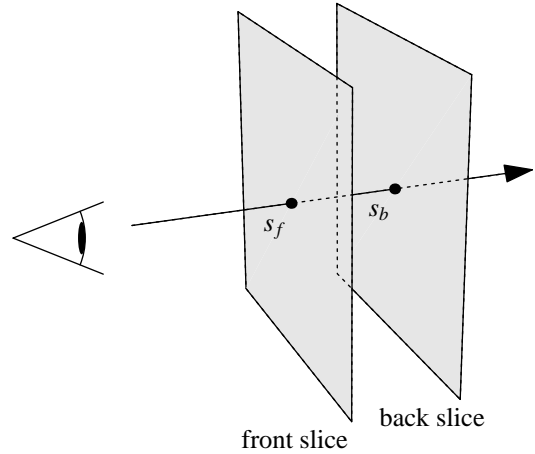
Figure 37: A slab of the volume between two slices. The scalar value on the front (back) slice for a particular viewing ray is called s_f ( s_b ).
