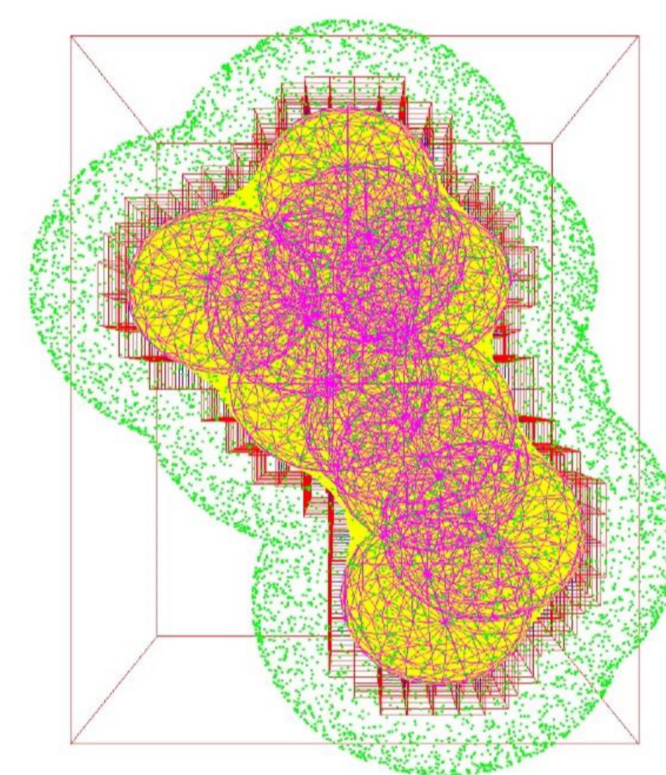
Figure 2: Illustration of structures used to calculate the SES for an example molecule with 10 atoms. The pink spheres are the atoms in space-filling representation, the green dots are the sample points sampling the SAS, the red boxes are the Marching Cubes and the yellow is the mesh generated as a result of running the Marching Cubes algorithm.
