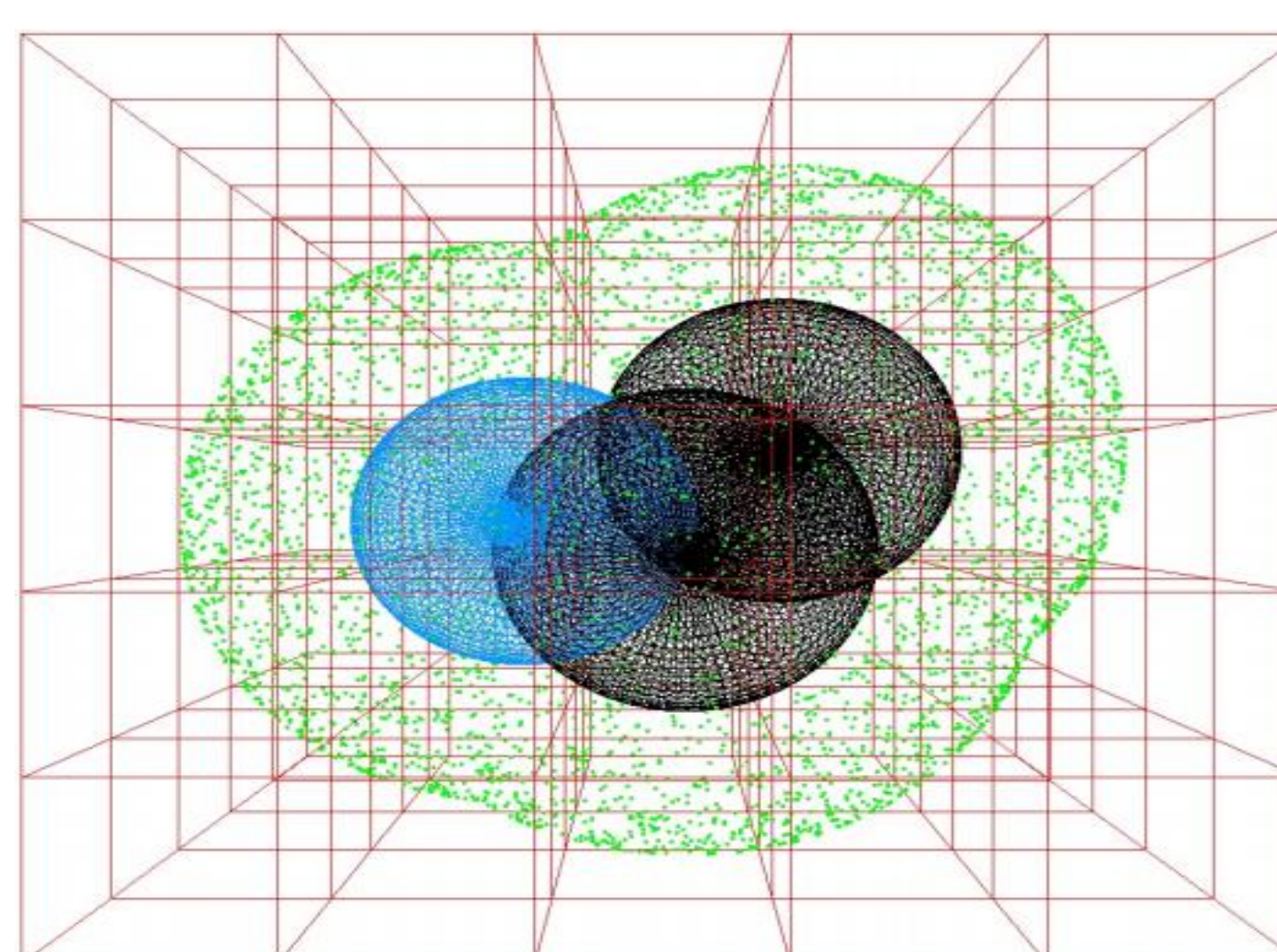
Figure 1: The green points are the sample points offset by 1.4 Å from the surface of the atoms. These points lie on the SAS. A test example of three atoms is shown. The spherical wireframe represents the atoms in space-filling model. The red boxes represent the regular grid containing the sample points.
