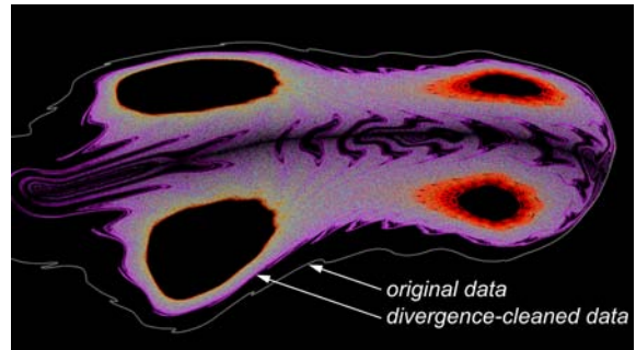
Figure 13: Unstable manifold computed in divergence-conserving interpolated field. Comparison of original data (white) and divergence-cleaned data (colored).
