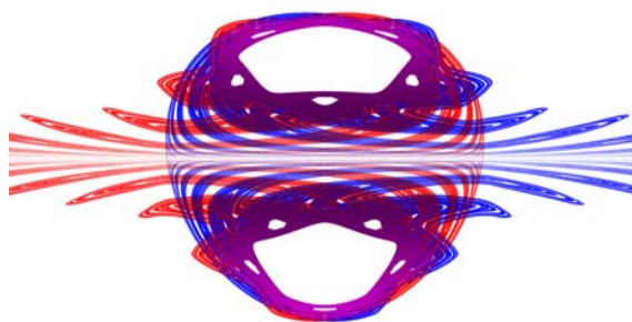
Figure 4: Manifolds of Figure 3 at longer integration time.
