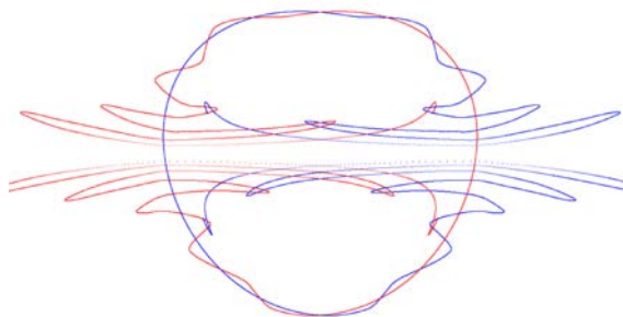
Figure 3: Planar section of 2D manifolds of a synthetic vortex breakdown bubble.
