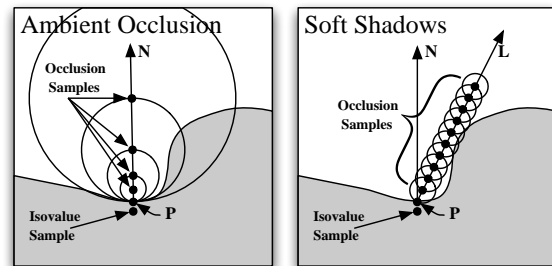
Figure 7: Illustration of our dynamic ambient occlusion and soft shadow algorithms. The isovalue is chosen one half of a voxel behind the isosurface. Ambient occlusion requires only 3-4 samples of different sizes in the direction of the surface normal. Soft shadows requires one ray cast in the direction of the light. In both cases the occlusion sample with the most occlusion is chosen.
