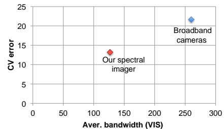
Figure 9: Bandwidth vs. radiometric accuracy.
