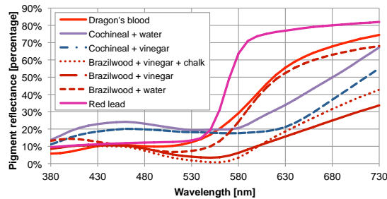
Figure 11: Measured reflectance of red candidate pigments.
