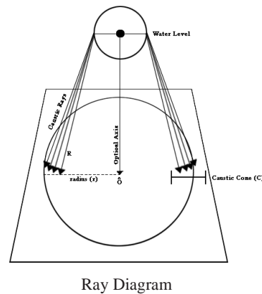
Figure 6: Ray diagram of a Caustic Cone. The lower rectangle represents the floor plane. The optical axis is defined by the vector from the light origin c in the \delta direction
