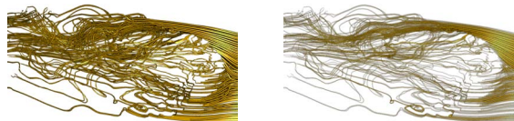
(a) 500 opaque path lines with 500 segments each, depth-dependent halos and 4x MSAA at 55fps. (b) Fragment linked lists with uniform transparency and standard blending. Achieves 26fps at 4x MSAA.
